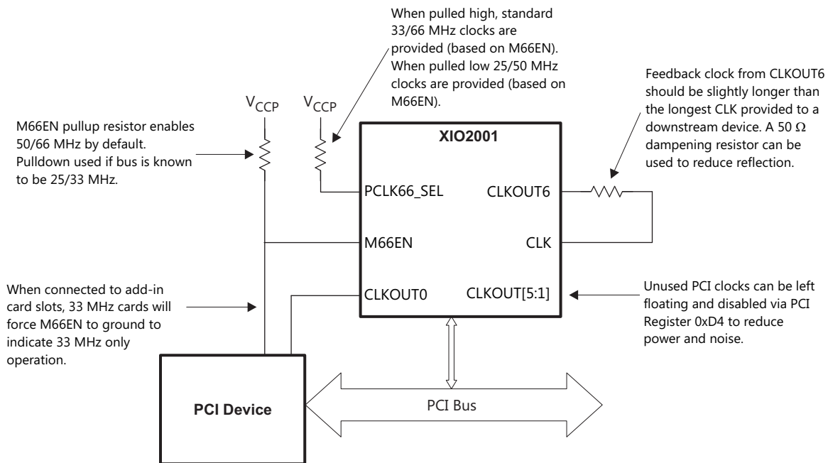
Figure 3. External PCI Bus Clock Configuration
