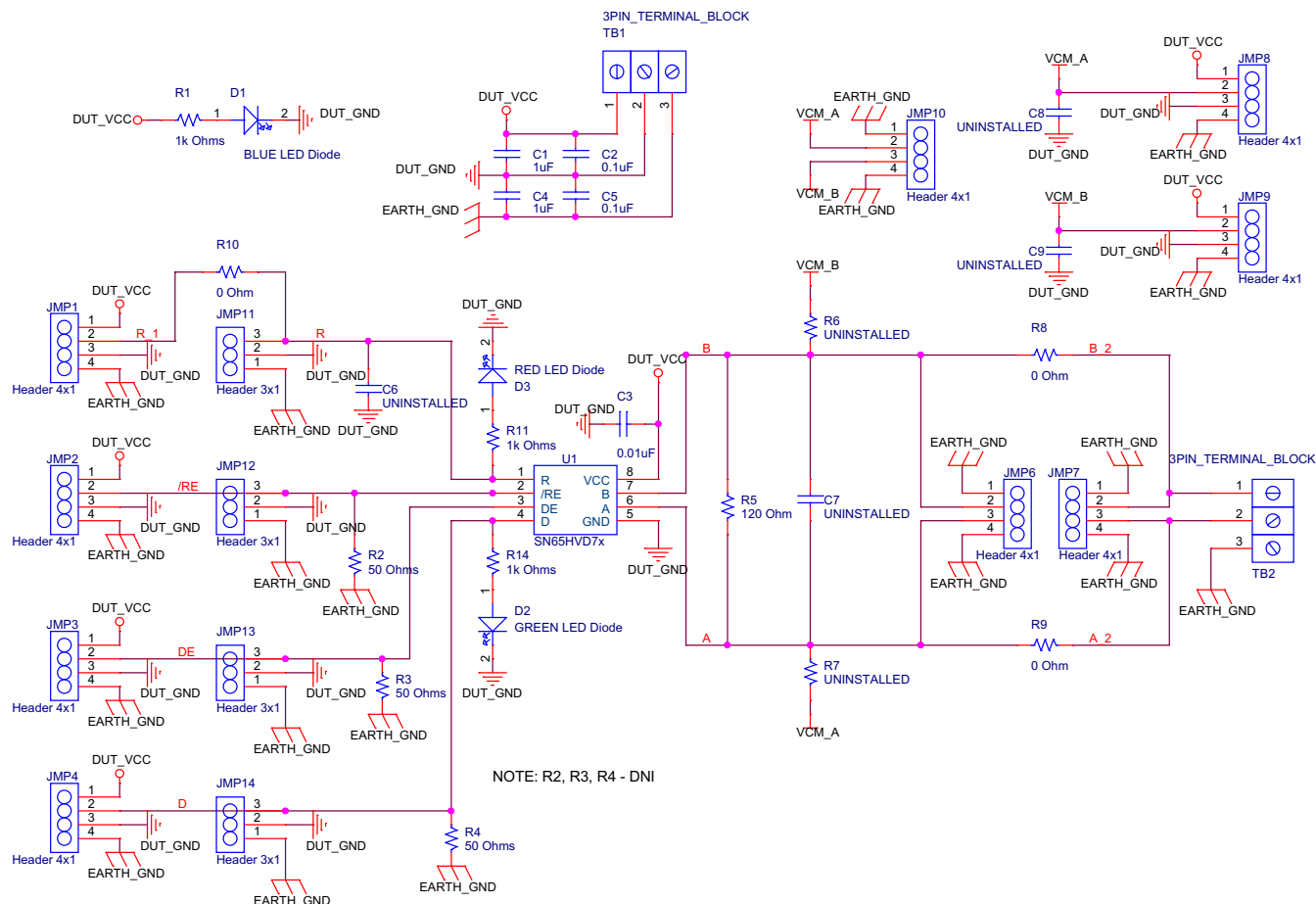
Figure 1. SN65HVD7xEVM Schematic
