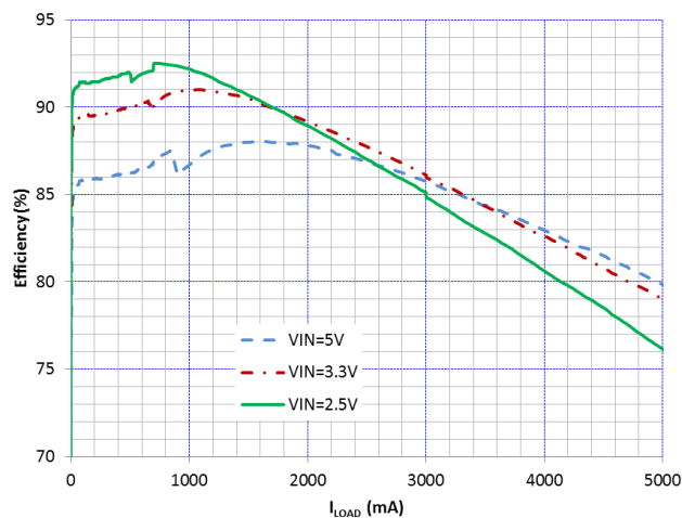
Figure 15. Efficiency vs I_{LOAD} and Temperature, V_{OUT} = 1.394\text{ V}
