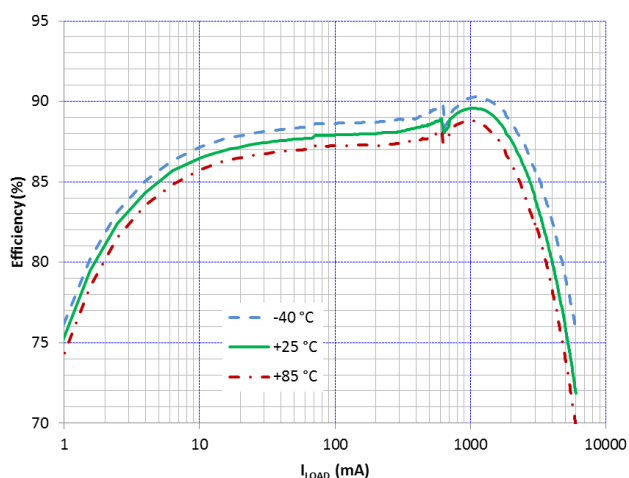
Figure 11. Efficiency vs I_{LOAD} and Temperature, V_{OUT} = 1.150\text{ V}
