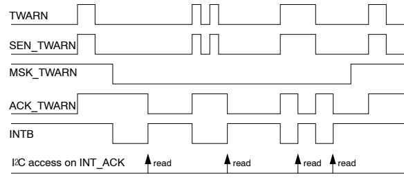
Figure 48. TWARN Interrupt Operation Example
