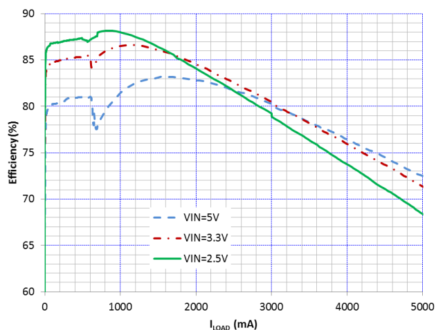
Figure 14. Efficiency vs I_{LOAD} and Temperature, V_{OUT} = 0.906\text{ V} , HEI201612A-R24M Inductor
