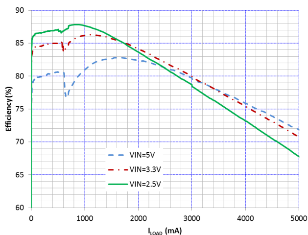
Figure 13. Efficiency vs I_{LOAD} and Temperature, V_{OUT} = 0.875\text{ V} , HEI201612A-R24M Inductor
