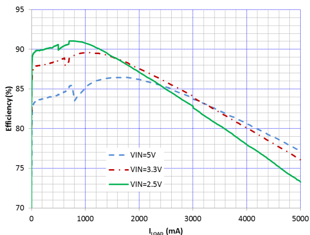
Figure 10. Efficiency vs I_{LOAD} and V_{IN} , V_{OUT} = 1.150\text{ V}
