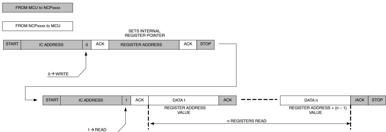
Figure 50. Read Sequence
