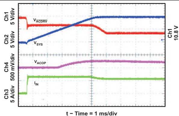
Figure 22. System Selector Learn Turnoff With 390 µF SYS-to-PGND System Capacitor
