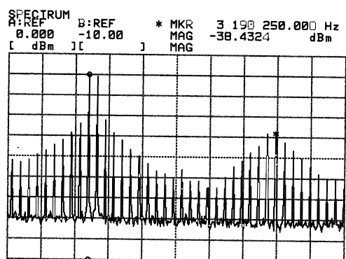
Figure 17. Inter-modulation Distortion Improvement
