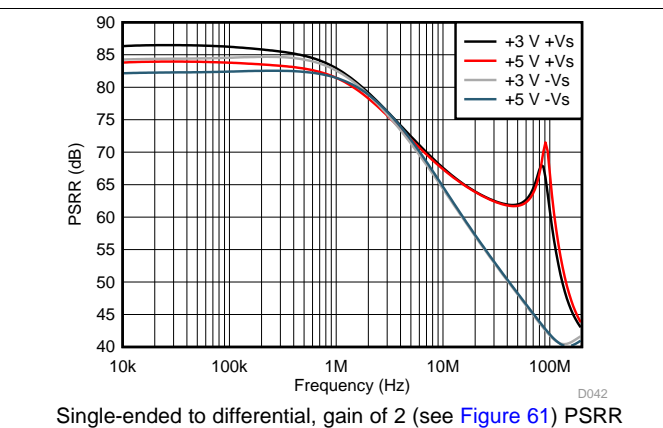
Figure 42. PSRR Over Frequency
