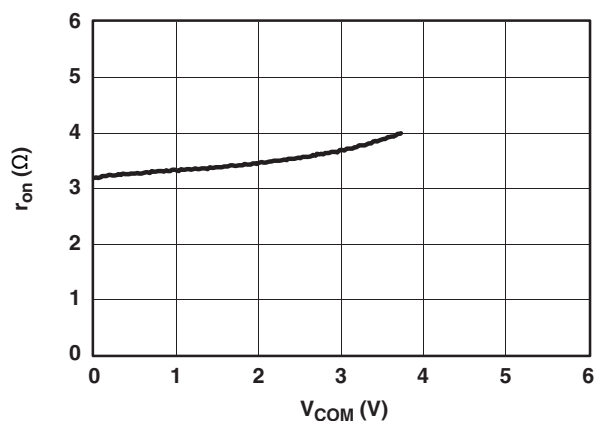
Figure 4. r on vs V COM (V CC = 3.6 V)
