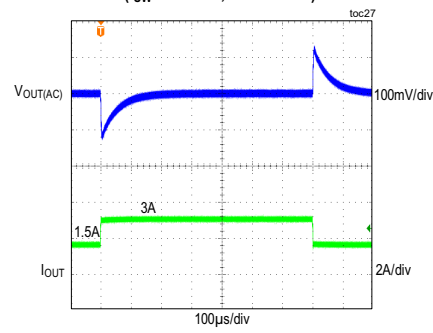
MAX17524, 5V OUTPUT LOAD TRANSIENT BETWEEN 1.5A AND 3A ( f_{SW} = 450kHz , PWM MODE)
