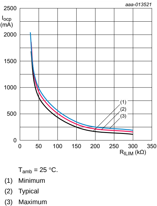
Fig 6. Typical overcurrent protection current versus the external resistor value
