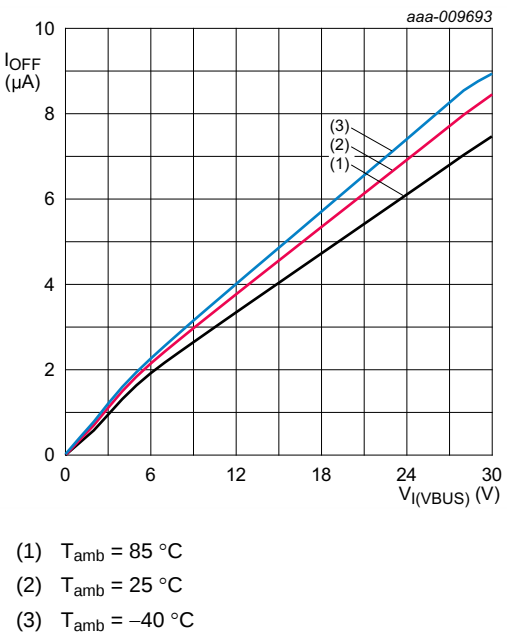
Fig 9. Typical power-off leakage current versus input voltage on pin VBUS
