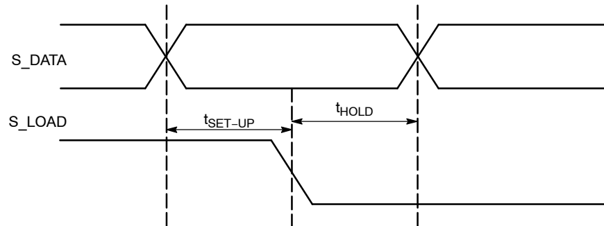
Figure 16. Setup and Hold
