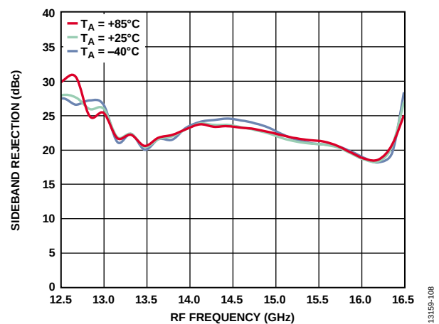
Figure 130. Sideband Rejection vs. RF Frequency at Various Temperatures, LO = 2 dBm, V_{DLOx} = 3.3 V
