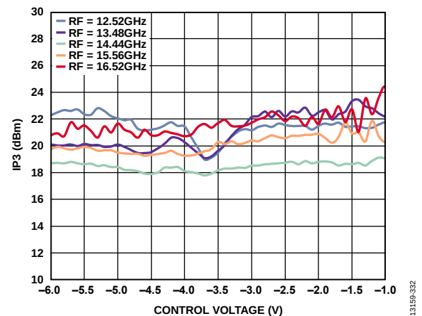
Figure 32. Input IP3 vs. Control Voltage at Various RF Frequencies, LO = 2 dBm, V_{DLOx} = 2.4V
