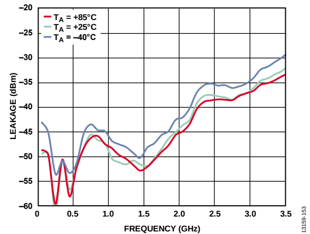
Figure 152. IF2 Leakage at RFOUT vs. Frequency at Various Temperatures, LO = 2 dBm
