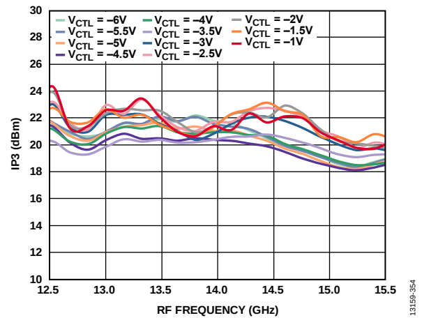
Figure 53. Input IP3 vs. RF Frequency at Various Control Voltages, LO = 2 dBm, V_{DLOx} = 2.4\text{ V}
