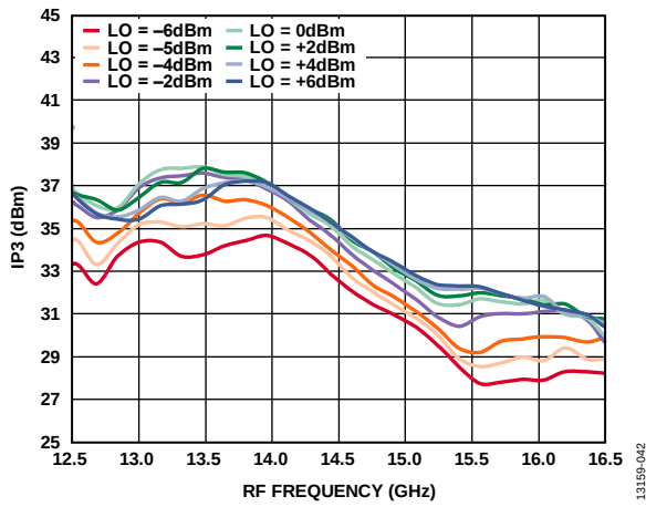
Figure 49. Output IP3 vs. RF Frequency at Various LO Powers, V_{DLOx} = 2.4\text{ V}
