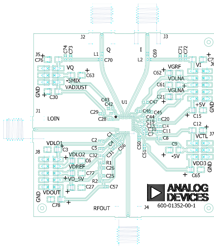
Figure 165. Evaluation Board Top Layer
