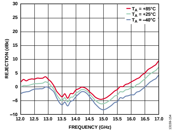
Figure 150. LO to RF Rejection vs. Frequency at Various Temperatures, LO = 2 dBm
