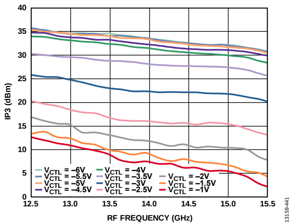
Figure 139. Output IP3 vs. RF Frequency at Various Control Voltages, LO = 2 dBm, V_{DLOX} = 3.3\text{ V}
