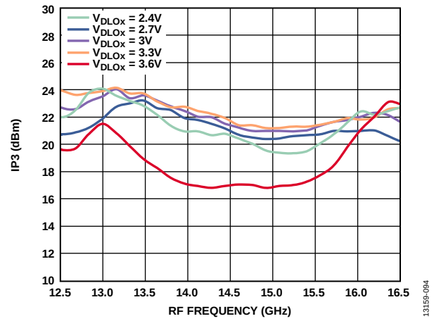
Figure 118. Input IP3 vs. RF Frequency at Various V_{DLOX} , LO = 2 dBm
