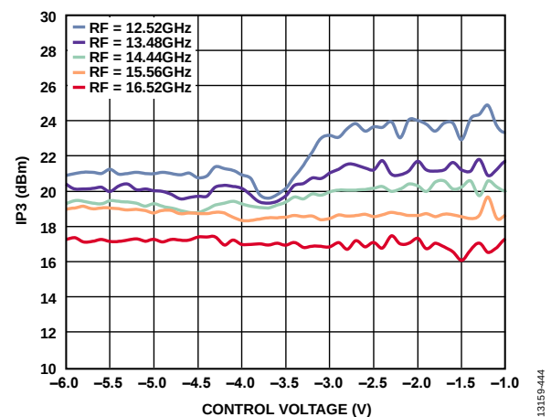
Figure 142. Input IP3 vs. Control Voltage at Various RF Frequencies, LO = 2 dBm, V_{DLOX} = 3.3\text{ V}
