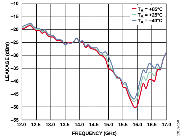
Figure 151. LO Leakage at IF2 vs. Frequency at Various Temperatures, LO = 2 dBm
