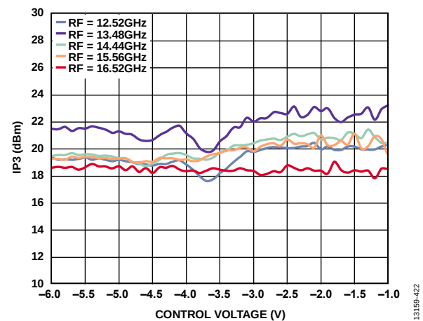
Figure 120. Input IP3 vs. Control Voltage at Various RF Frequencies, LO = 2 dBm, V_{DLOX} = 3.3\text{ V}
