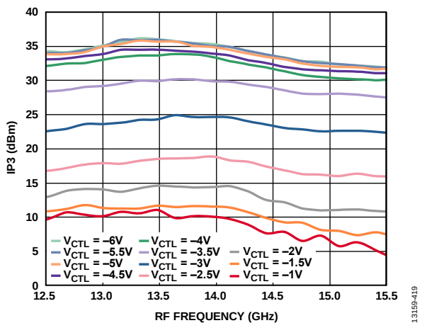
Figure 117. Output IP3 vs. RF Frequency at Various Control Voltages, LO = 2 dBm, V_{DLOX} = 3.3\text{ V}
