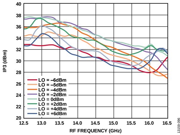
Figure 115. Output IP3 vs. RF Frequency at Various LO Powers, V_{DLOX} = 3.3\text{ V}
