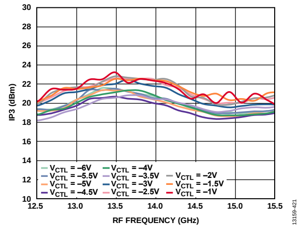
Figure 119. Input IP3 vs. RF Frequency at Various Control Voltages, LO = 2 dBm, V_{DLOX} = 3.3\text{ V}
