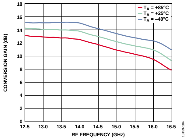
Figure 125. Conversion Gain vs. RF Frequency at Various Temperatures, LO = 2 dBm, V_{DLO1} = 3.3 V
