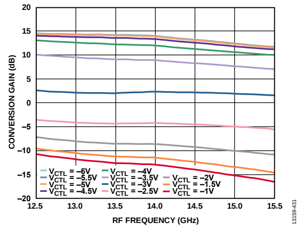
Figure 129. Conversion Gain vs. RF Frequency at Various Control Voltages, LO = 2 dBm, V_{DLOx} = 3.3 V
