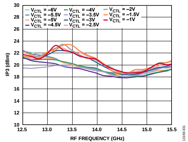
Figure 31. Input IP3 vs. RF Frequency at Various Control Voltages, LO = 2 dBm, V_{DLOx} = 2.4V
