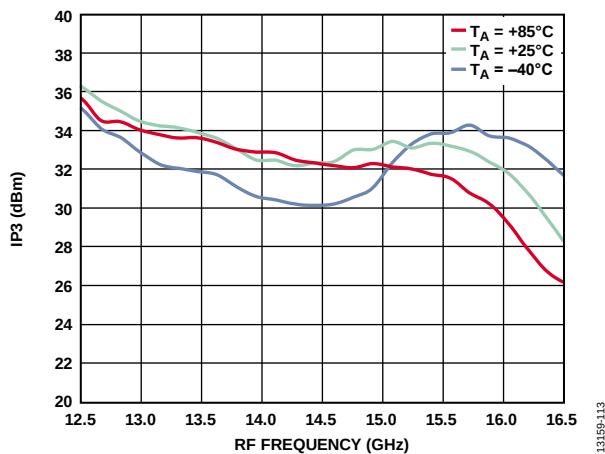
Figure 133. Output IP3 vs. RF Frequency at Various Temperatures, LO = 2 dBm, V_{DLOX} = 3.3 V
