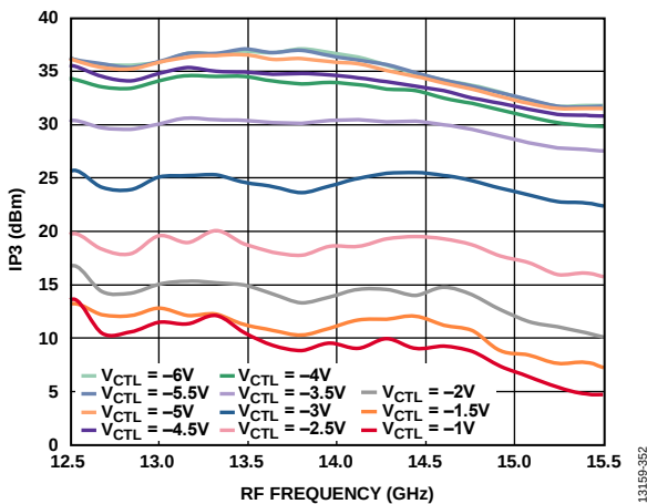
Figure 51. Output IP3 vs. RF Frequency at Various Control Voltages, LO = 2 dBm, V_{DLOx} = 2.4\text{ V}
