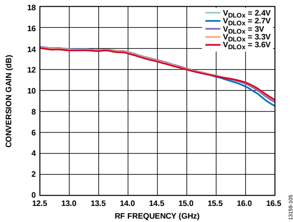
Figure 126. Conversion Gain vs. RF Frequency at Various V_{DLOx} , LO = 2 dBm
