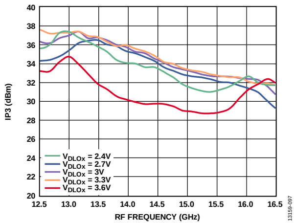
Figure 116. Output IP3 vs. RF Frequency at Various V_{DLOX} , LO = 2 dBm
