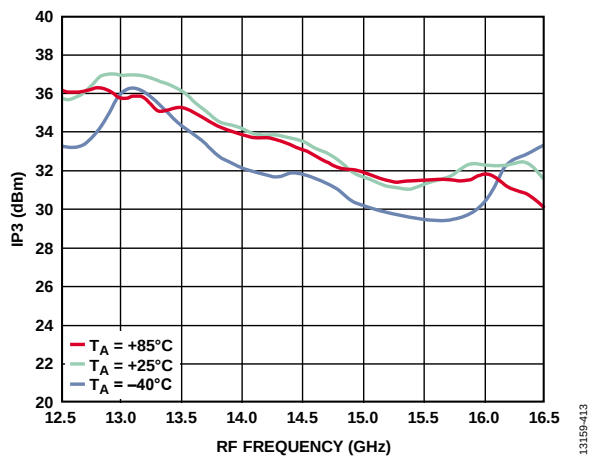
Figure 111. Output IP3 vs. RF Frequency at Various Temperatures, LO = 2 dBm, V_{DLOX} = 3.3\text{ V}
