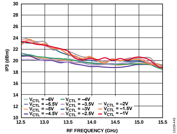
Figure 141. Input IP3 vs. RF Frequency at Various Control Voltages, LO = 2 dBm, V_{DLOX} = 3.3\text{ V}
