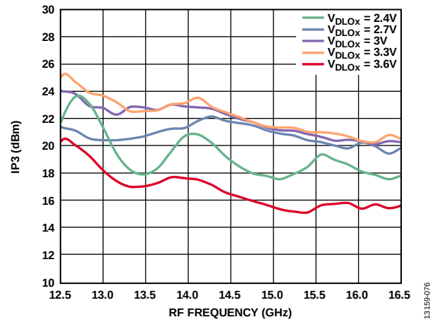
Figure 96. Input IP3 vs. RF Frequency at Various V_{DLOx} , LO = 2 dBm
