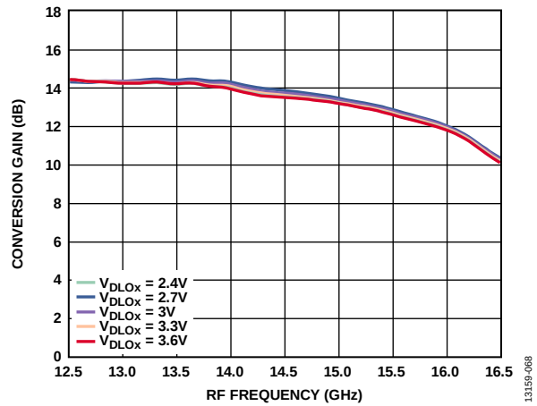
Figure 82. Conversion Gain vs. RF Frequency at Various V_{DLOx} , LO = 2 dBm
