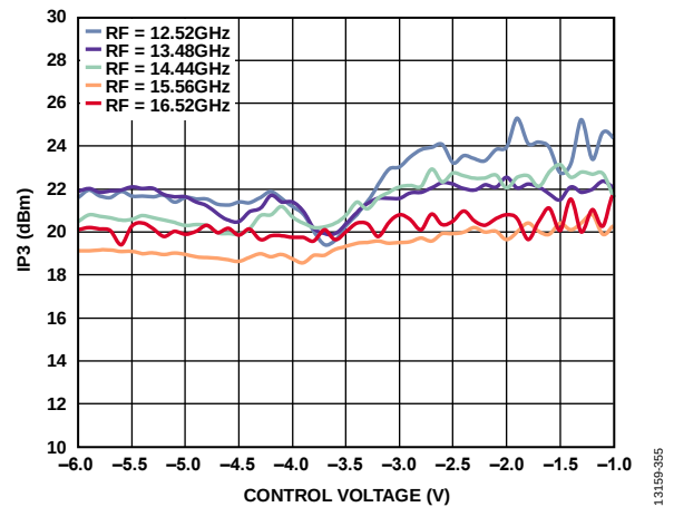
Figure 54. Input IP3 vs. Control Voltage at Various RF Frequencies, LO = 2 dBm, V_{DLOx} = 2.4\text{ V}
