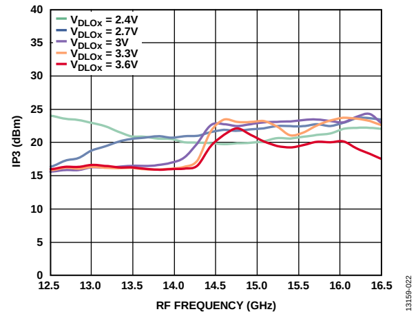
Figure 30. Input IP3 vs. RF Frequency at Various V_{DLOx} , LO = 2 dBm
