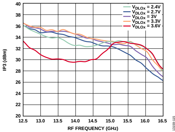
Figure 138. Output IP3 vs. RF Frequency at Various V_{DLOX} , LO = 2 dBm
