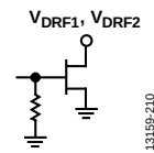
Figure 10. V_{DRF1} , V_{DRF2} Interface
