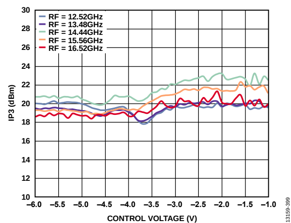
Figure 98. Input IP3 vs. Control Voltage at Various RF Frequencies, LO = 2 dBm, V_{DLOx} = 3.3\text{ V}
