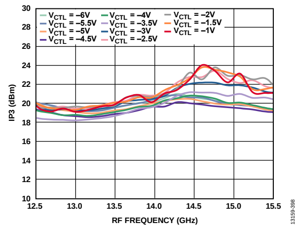
Figure 97. Input IP3 vs. RF Frequency at Various Control Voltages, LO = 2 dBm, V_{DLOx} = 3.3\text{ V}
