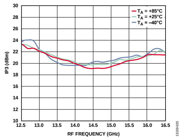
Figure 25. Input IP3 vs. RF Frequency at Various Temperatures, LO = 2 dBm, V_{DLOx} = 2.4 V
