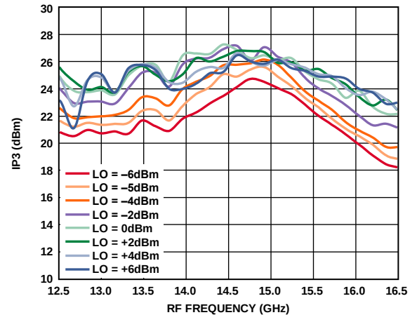
Figure 70. Input IP3 vs. RF Frequency at Various LO Powers, V_{DLOx} = 2.4 V
