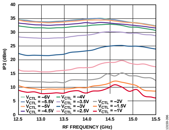
Figure 95. Output IP3 vs. RF Frequency at Various Control Voltages, LO = 2 dBm, V_{DLOx} = 3.3\text{ V}
