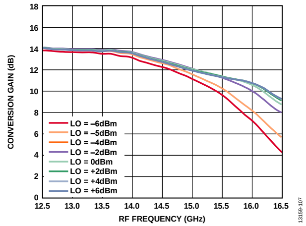
Figure 128. Conversion Gain vs. RF Frequency at Various LO Powers, V_{DLOx} = 3.3 V
