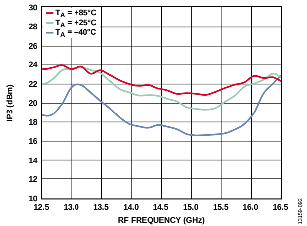
Figure 113. Input IP3 vs. RF Frequency at Various Temperatures, LO = 2 dBm, V_{DLOX} = 3.3\text{ V}
