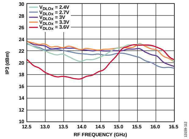
Figure 140. Input IP3 vs. RF Frequency at Various V_{DLOX} , LO = 2 dBm
