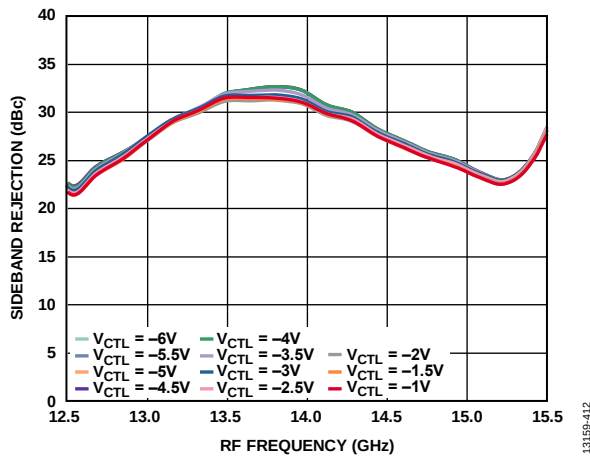
Figure 110. Sideband Rejection vs. RF Frequency at Various Control Voltages, LO = 2 dBm, V_{DLOX} = 3.3\text{ V}
