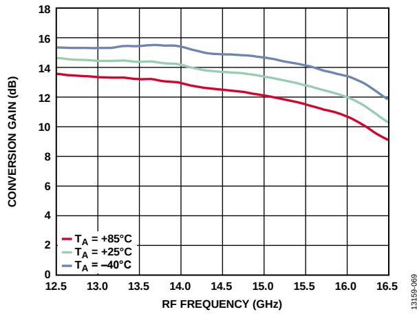
Figure 81. Conversion Gain vs. RF Frequency at Various Temperatures, LO = 2 dBm, V_{DLOx} = 3.3 V
