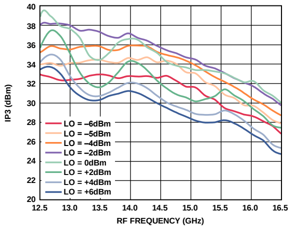
Figure 93. Output IP3 vs. RF Frequency at Various LO Powers, V_{DLOx} = 3.3\text{ V}
