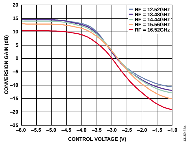
Figure 83. Conversion Gain vs. Control Voltage at Various RF Frequencies, LO = 2 dBm, V_{DLOx} = 3.3 V
