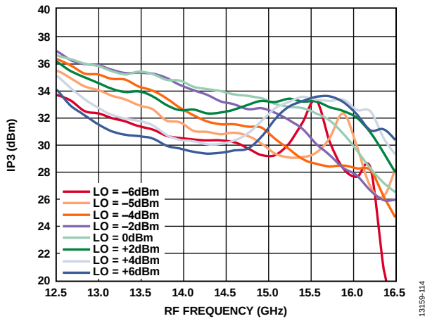
Figure 137. Output IP3 vs. RF Frequency at Various LO Powers, V_{DLOX} = 3.3\text{ V}
