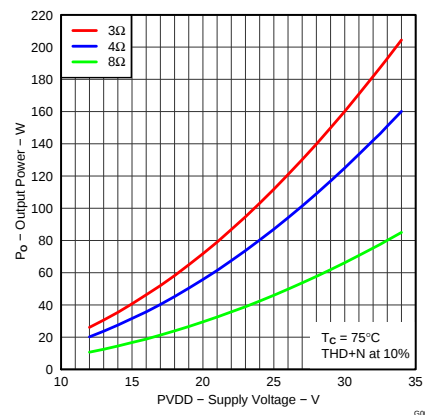
Figure 18. Output Power vs Supply Voltage vs Distortion + Noise = 10%
