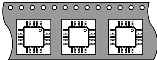
Figure 10. LQFP, TQFP
