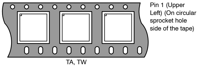
Figure 43. DFN/QFN (LPCC)/ WLCSP-4/XDFN2
