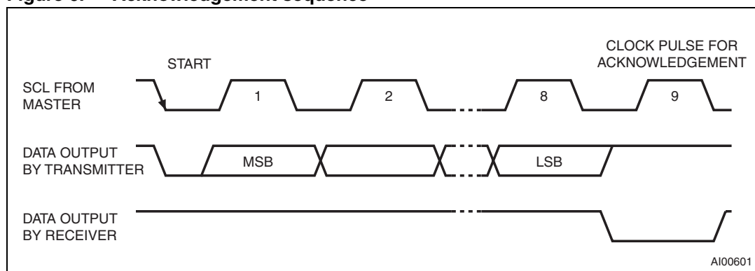
Figure 6. Acknowledgement sequence
