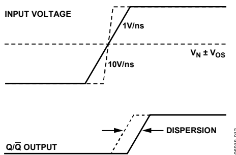
Figure 13. Propagation Delay—Slew Rate Dispersion
