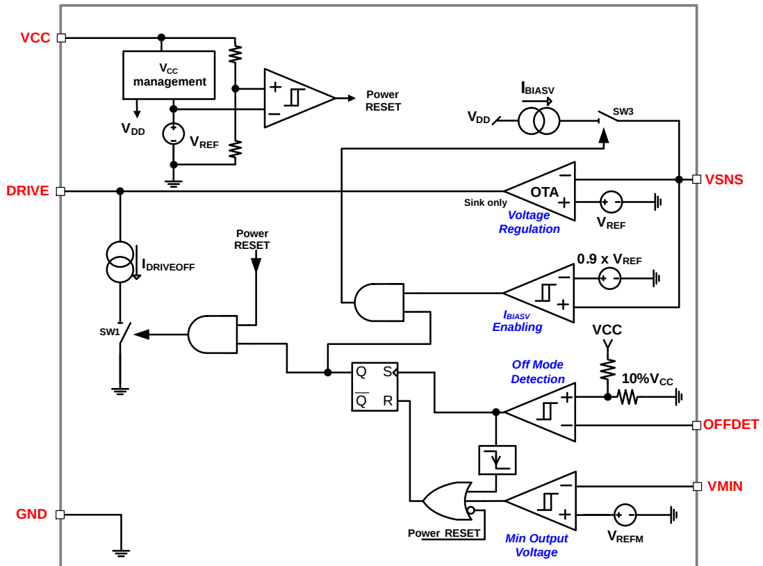
NCP4353B
