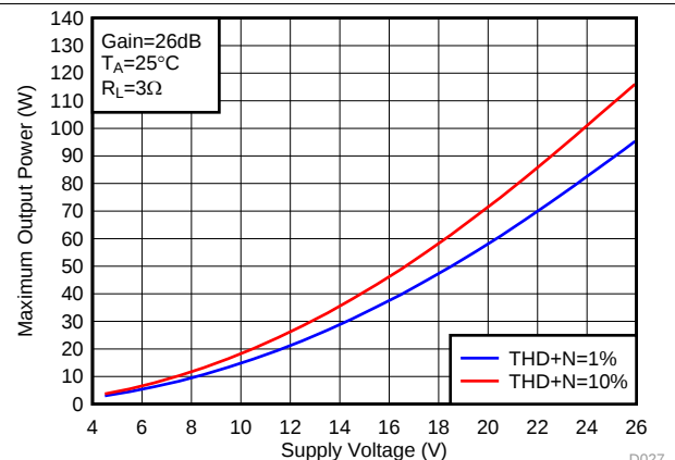
Figure 24. Maximum Output Power (PBTL) vs Supply Voltage
