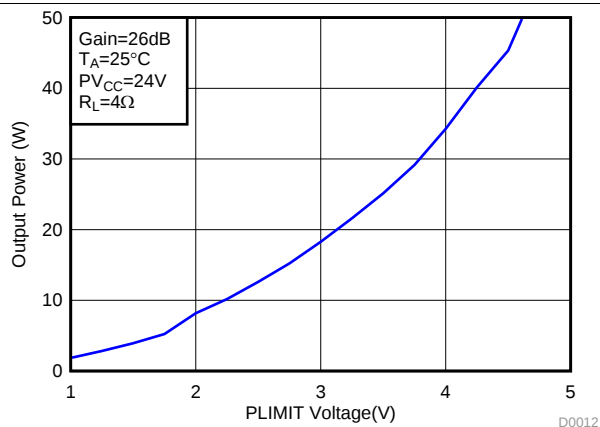
Figure 9. Output Power (BTL) vs Plimit Voltage
