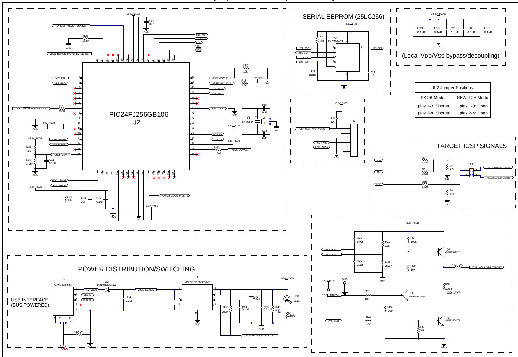
FIGURE A-6: PIC32MZ EMBEDDED CONNECTIVITY (EC) STARTER KIT (DEBUGGER)
