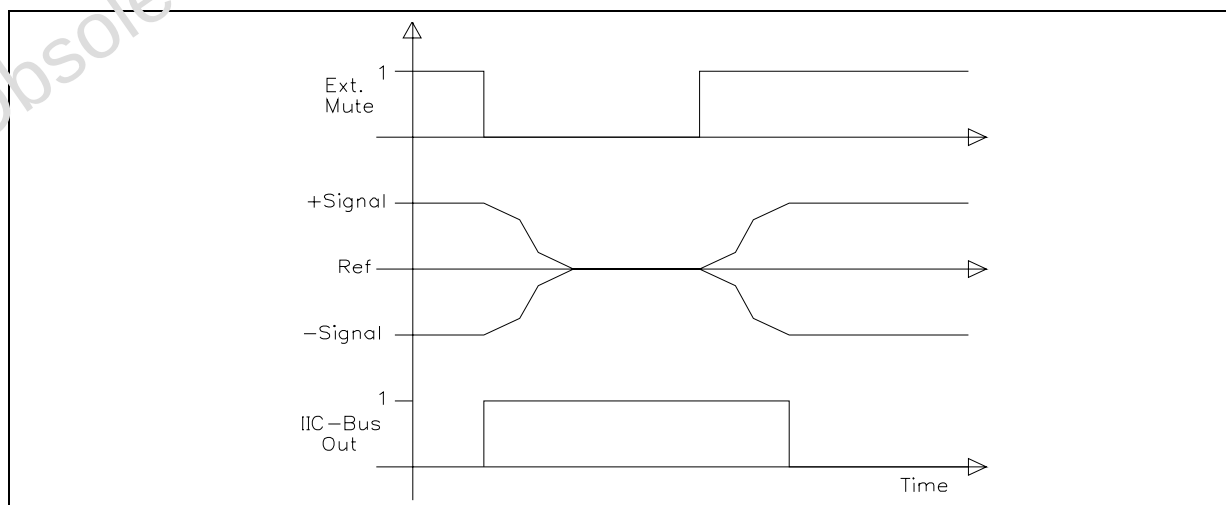
Figure 6. Softmute-Timing
