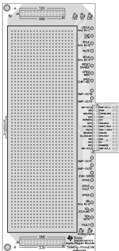
Figure 6. Top Overlay
