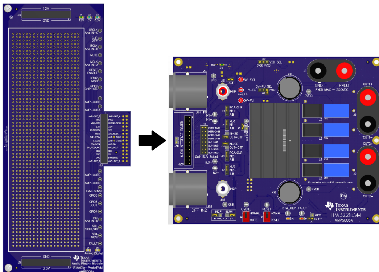
Figure 3. Connecting Prototype Plug-in Module to EVM
