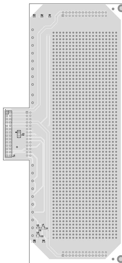
Figure 7. Bottom Overlay
