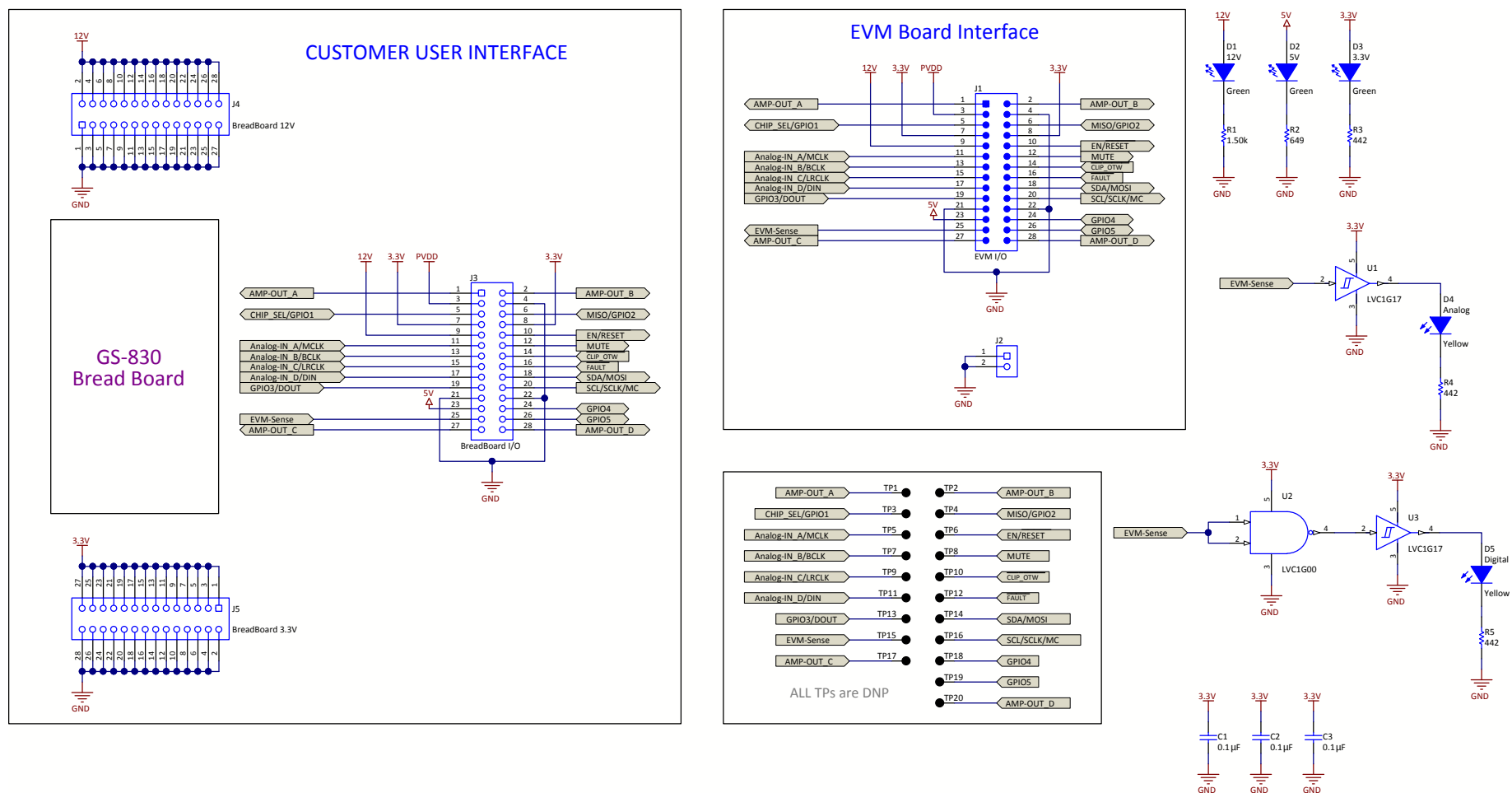
Figure 5. SIDEIG-PROTOEVM Schematic
