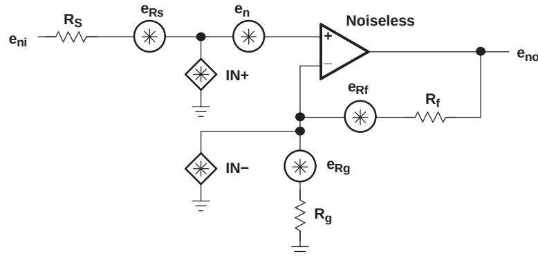
Figure 78. Noise Model
