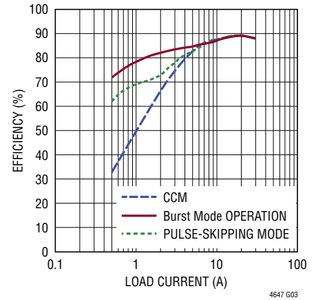
CCM, Burst Mode and Pulse-Skipping Mode Efficiency V_{IN} = 12V , V_{OUT} = 1.2V , 500kHz
