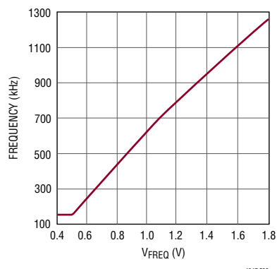
Figure 2. Relationship Between Switching Frequency and FREQ Pin Voltage
