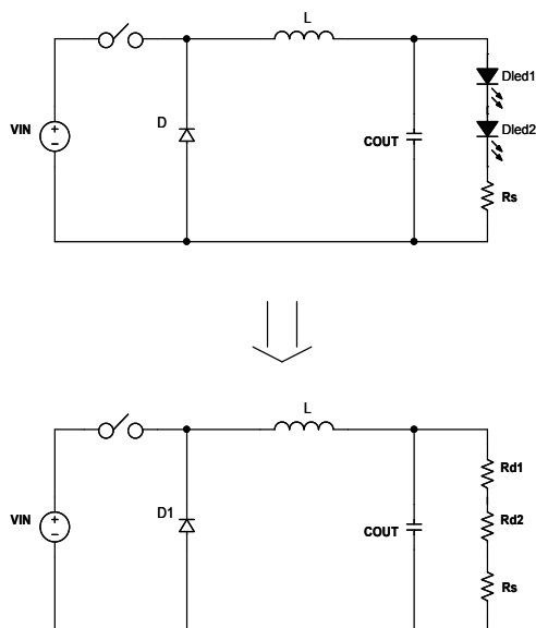
Figure 8. Load equivalent circuit
