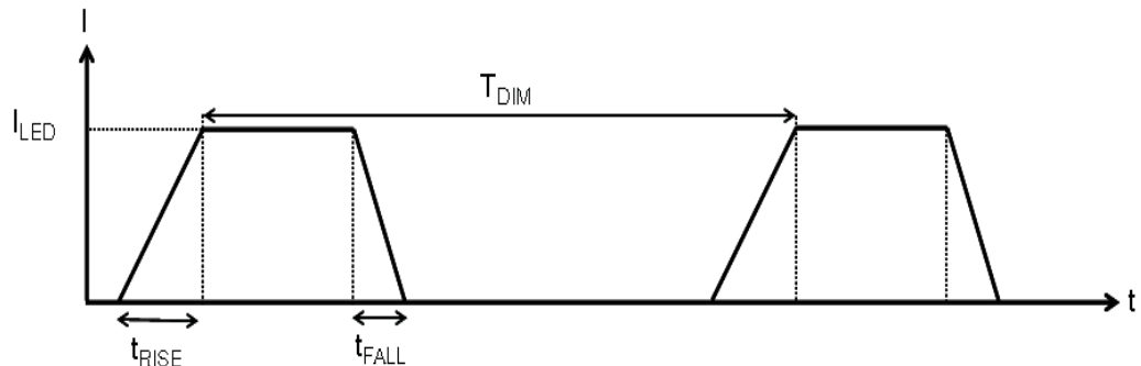
Figure 13. Dimming signal
