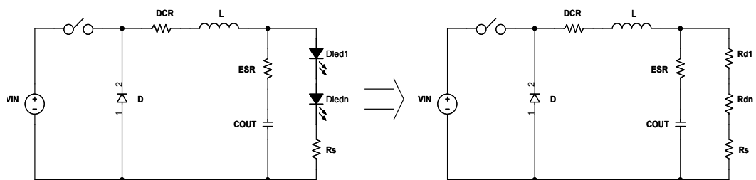
Figure 15. Equivalent circuit
