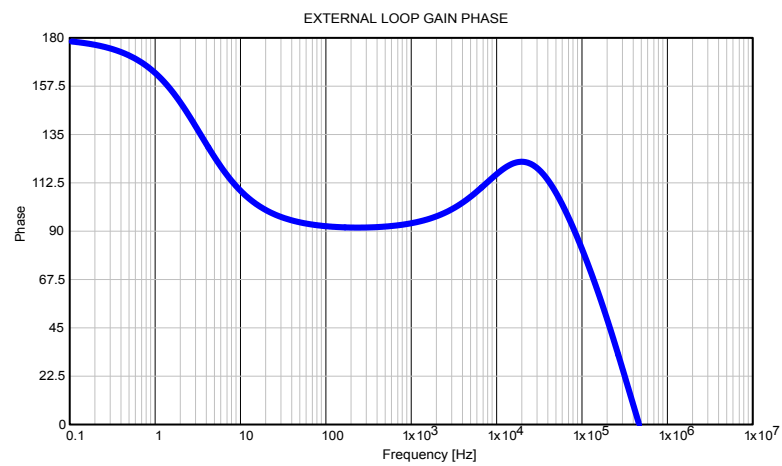
Figure 10. Phase plot
