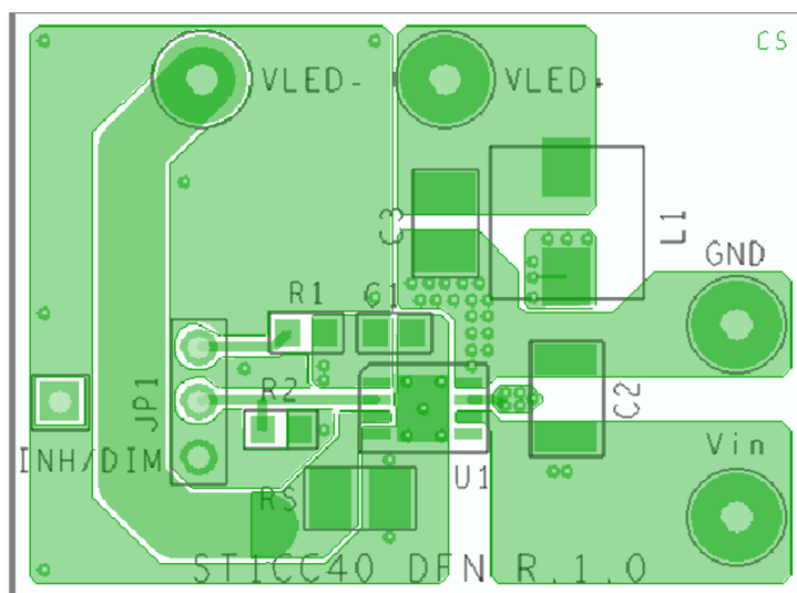
Figure 20. PCB layout (component side) DFN package
