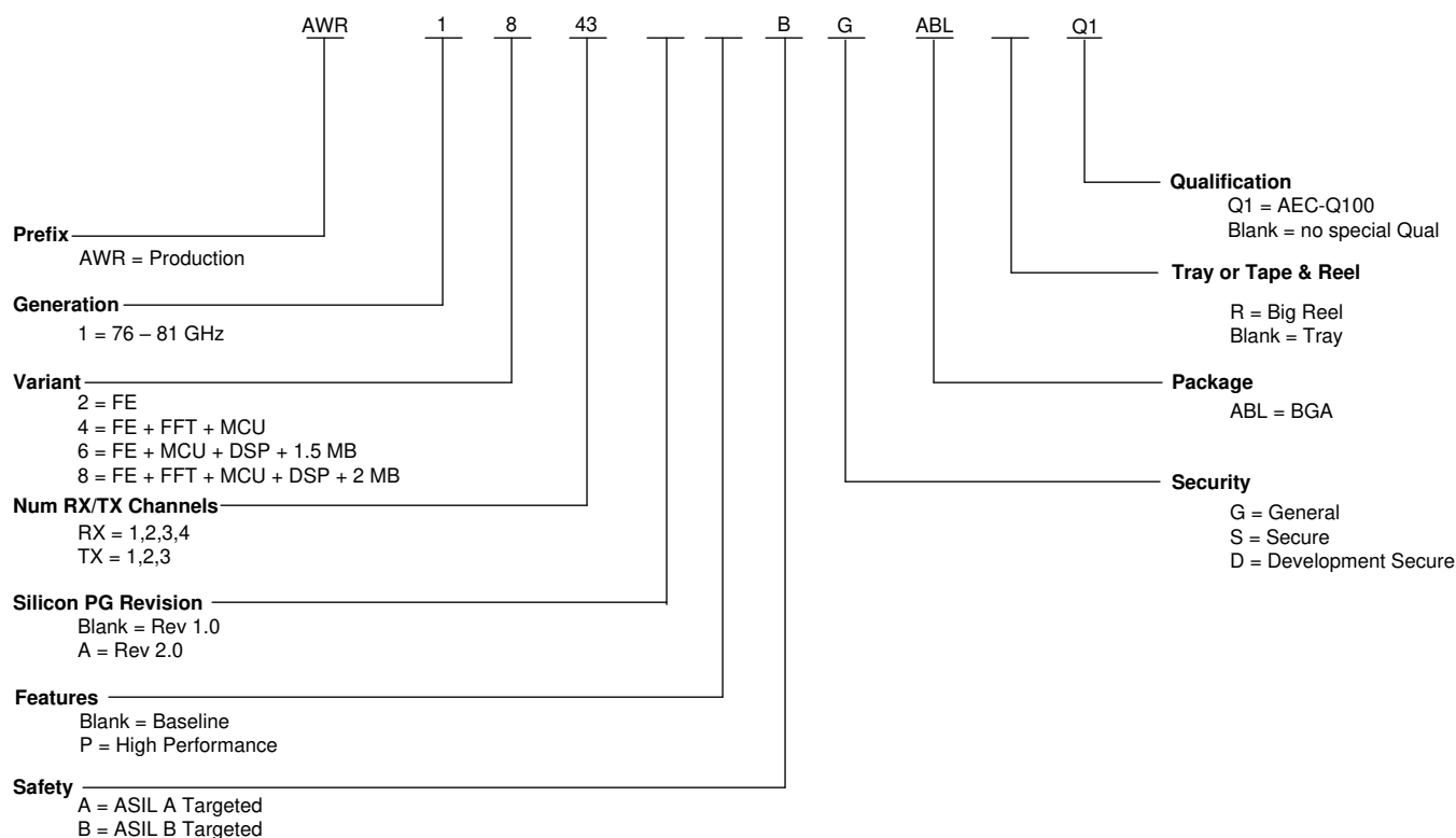
Figure 9-1. Device Nomenclature
