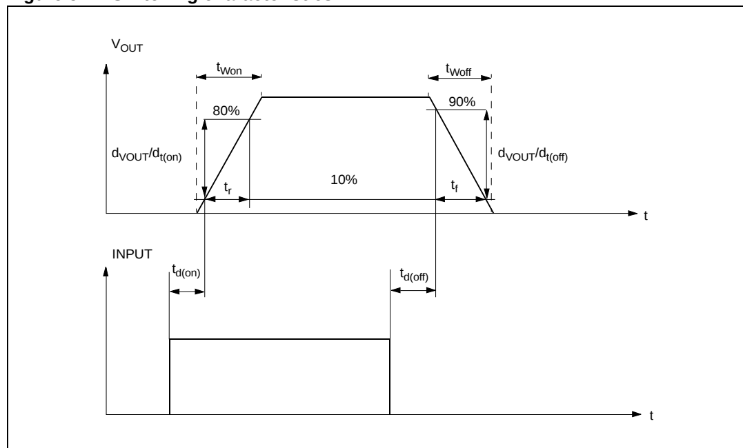
Figure 5. Switching characteristics
