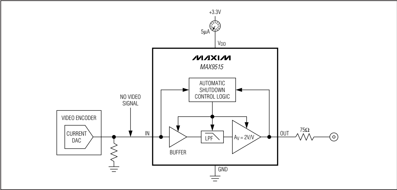
Figure 1. Automatic Shutdown
