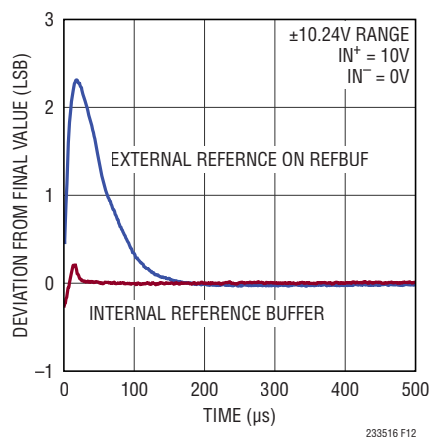
Figure 12. Burst Conversion Response of the LTC2335-16, f_{\text{SMPL}} = 1\text{Msps}
