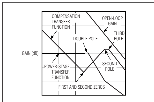
Figure 4. Type III Compensation Illustration
