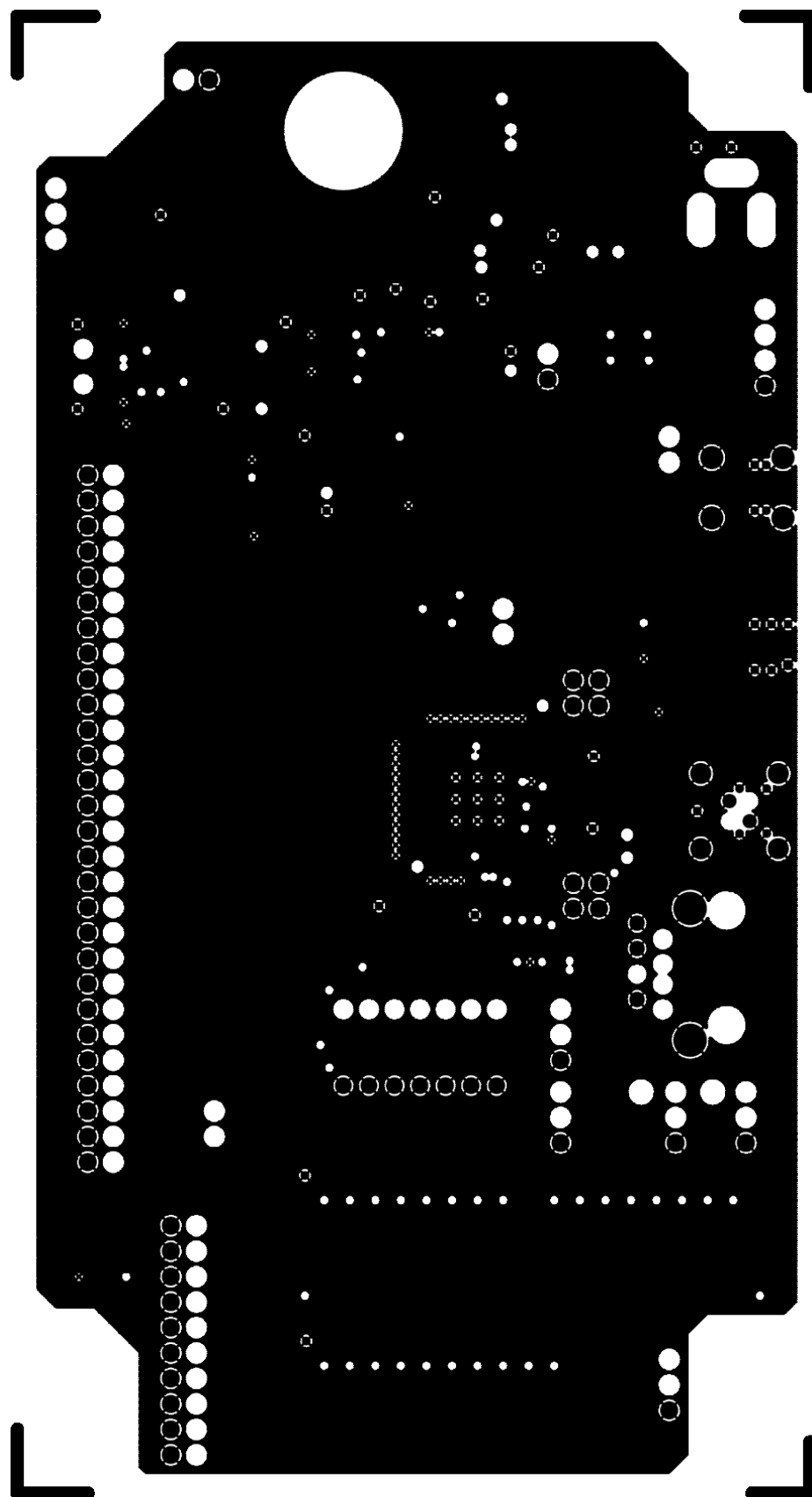
Figure 7: GND Layer
