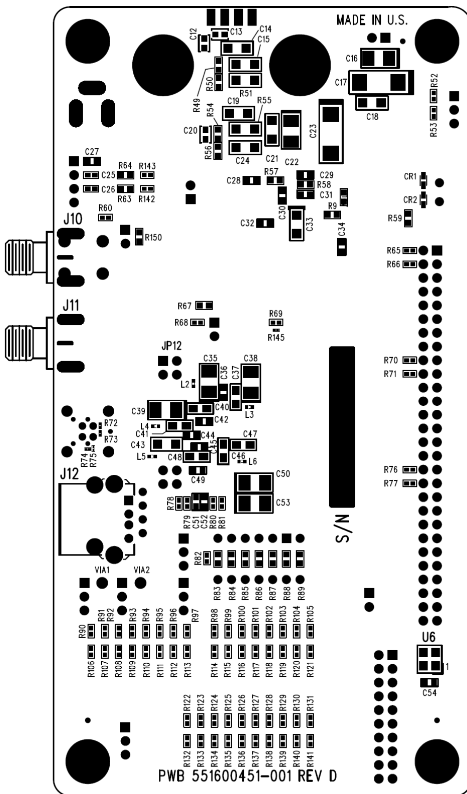
Figure 5: BOTTOM View
