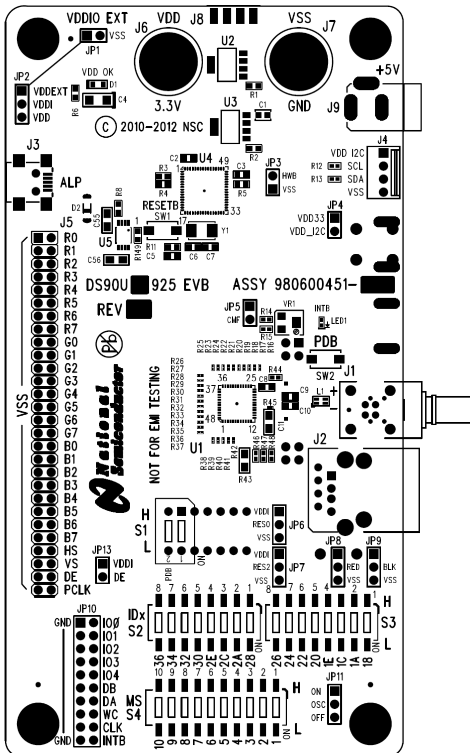
Figure 4: TOP View
