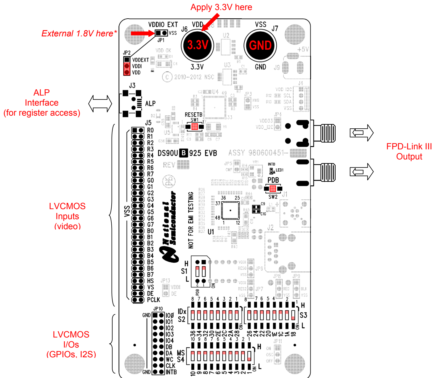
Figure 1: DS90UB925Q EVB
