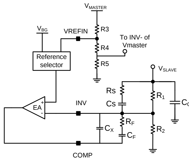
Figure 6. Co-incident Tracking Circuit Connections
