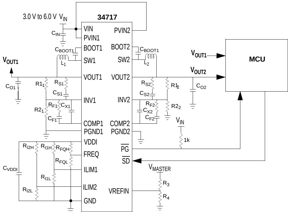
Figure 1. Application diagram for 34717
