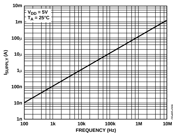
Figure 6. Supply Current vs. Input Switching Frequency
