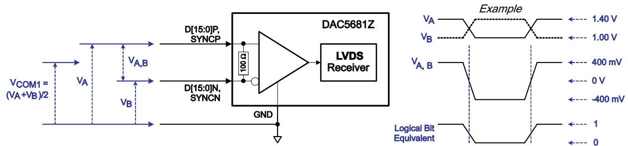
Figure 31. LVDS Data (D[15:0]P/N, SYNCN/P Pairs) Input Levels
