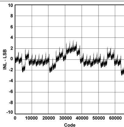
Figure 1. Integral Nonlinearity
