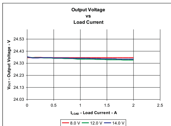
Figure 6. TPS40210EVM Output Voltage vs Load Current ( V_{IN} = 8 V to 14 V, V_{OUT} = 24.0 V, I_{OUT} = 0 A to 2 A)
