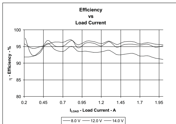
Figure 5. TPS40210EVM Efficiency vs. Load Current ( V_{IN} = 8 V to 14 V, V_{OUT} = 24.0 V, I_{OUT} = 0 A to 2 A)
