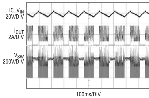
Figure 11. V_{IN} = 270VAC
