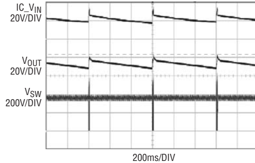
Figure 9. V_{IN} = 270VAC
