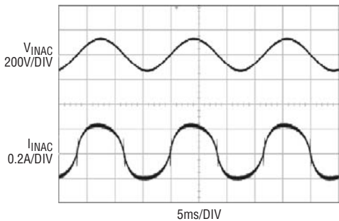
Figure 4. V IN = 90VAC
