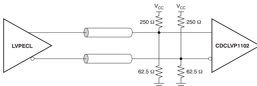
Figure 16. DC-Coupled LVPECL Inputs to CDCLVP1102 ( V_{CC} = 2.5 V)
