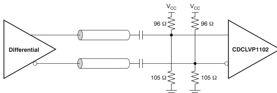
Figure 18. AC-Coupled Differential Inputs to CDCLVP1102 ( V_{CC} = 2.5 V)
