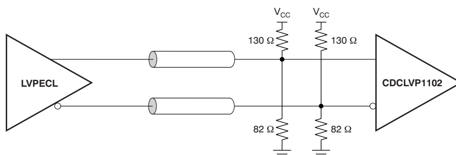
Figure 17. DC-Coupled LVPECL Inputs to CDCLVP1102 ( V_{CC} = 3.3 V)
