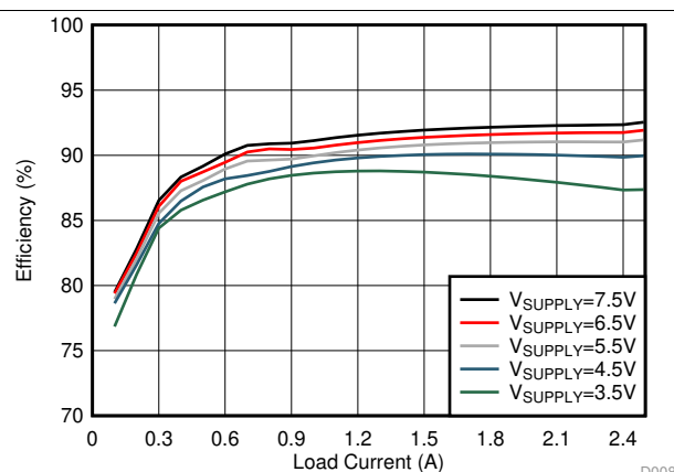
Figure 8. Efficiency vs Load Current ( V_{LOAD} = 9.5\text{ V} , F_{SW} = 440\text{ kHz} , SS Configuration)
