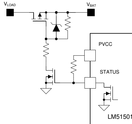
Figure 18. Disconnection Switch Control Example
