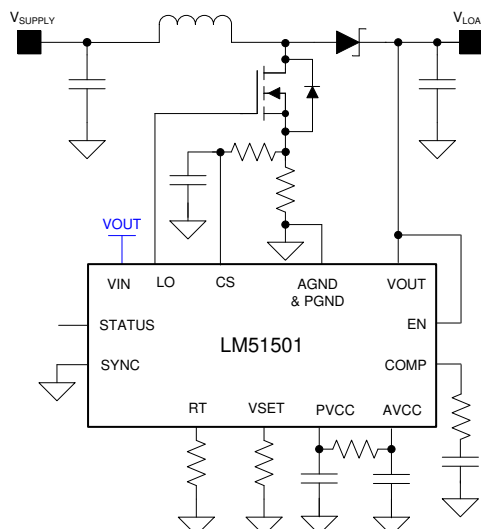
Figure 22. Lower Standby Threshold in SS Configuration
