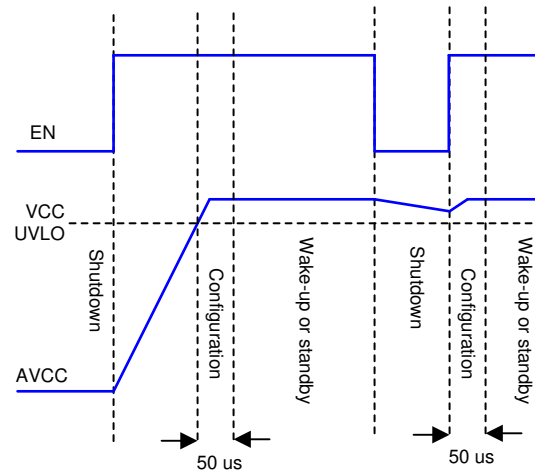
Figure 9. Power-On Voltage Selection
