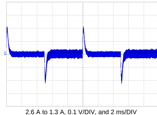
Figure 21. Load Transient
