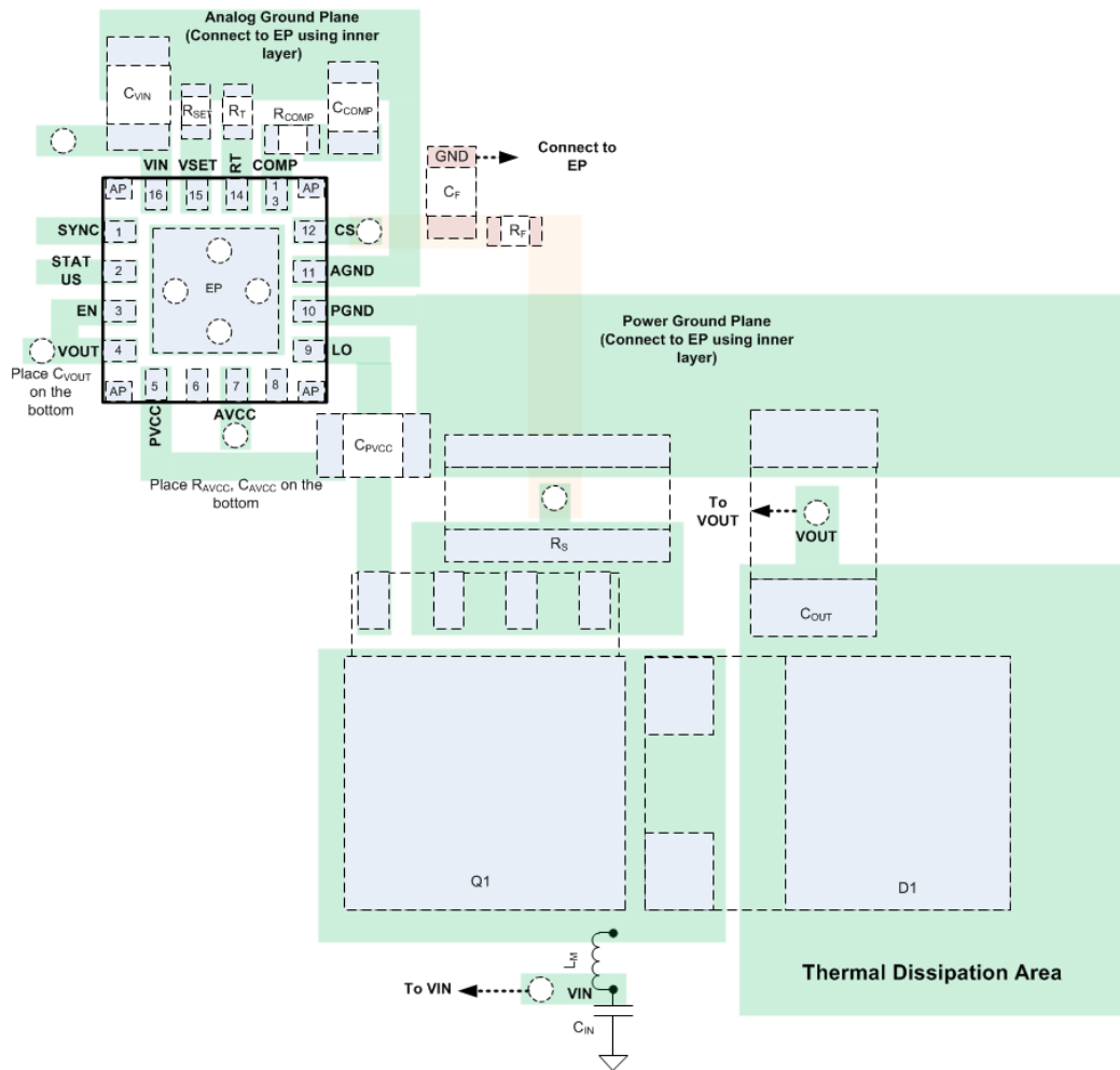
Figure 27. LM51501-Q1 PCB Layout Example
