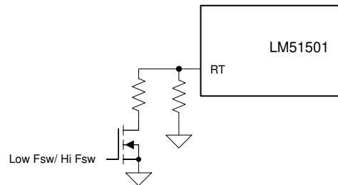
Figure 25. Dynamic Frequency Change
