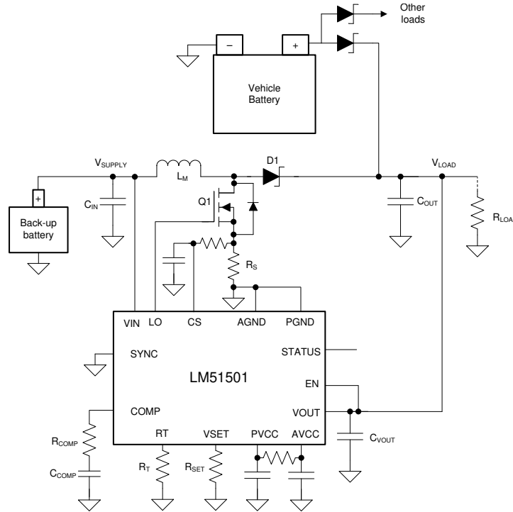
Figure 16. Typical Emergency Call Application
