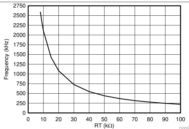
Figure 5. Frequency vs RT
