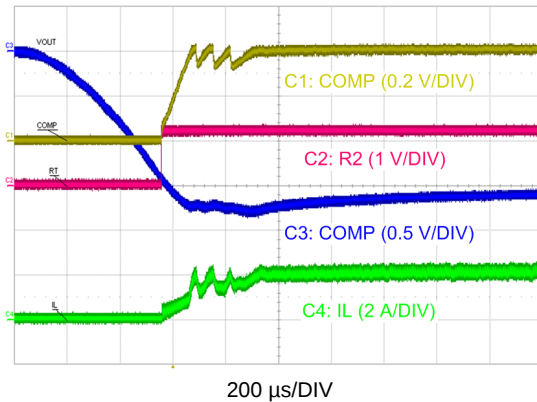
Figure 20. Automatic Wake-Up
