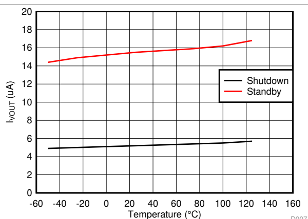
Figure 7. I_{VOUT} vs Temperature
