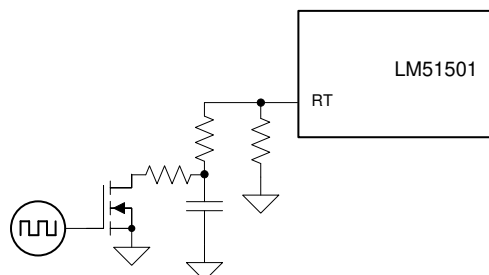
Figure 26. Dithering Using an External Clock
