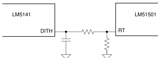
Figure 23. Dithering Using the Dither-Enabled Device LM5141
