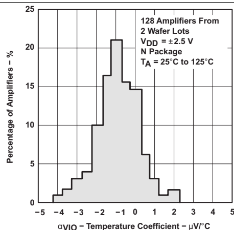
Figure 10. Distribution of TLC2274-Q1 vs Input Offset Voltage Temperature Coefficient
