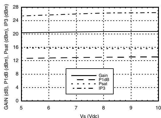
Gain, Power & OIP3 vs. Supply Voltage for Constant I_{CC} = 35 \text{ mA} @ 850 MHz
