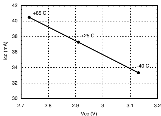
I_{CC} vs. V_{CC} Over Temperature for Fixed V_S = 5V , R_{BIAS} = 56 \text{ Ohms}
