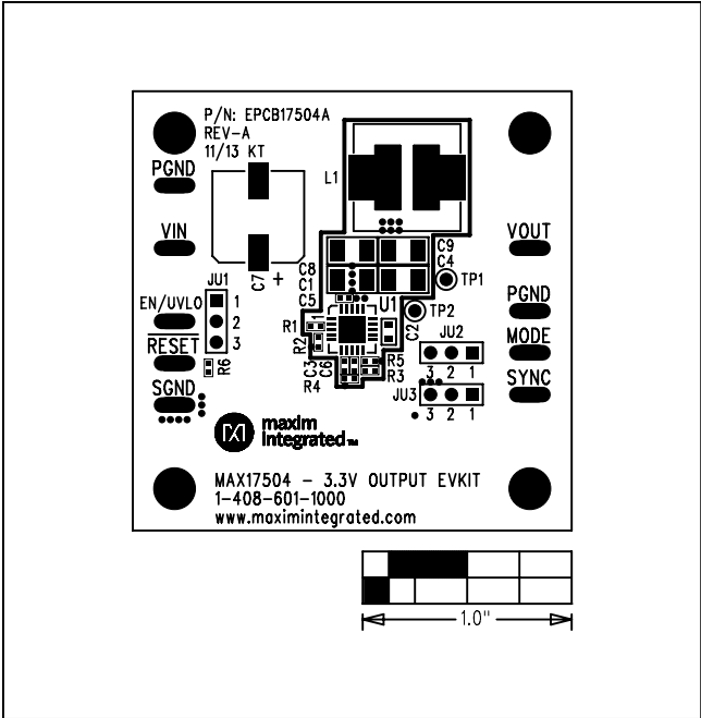
Figure 12. MAX17504 3.3V Output EV Kit Component Placement Guide—Component Side
