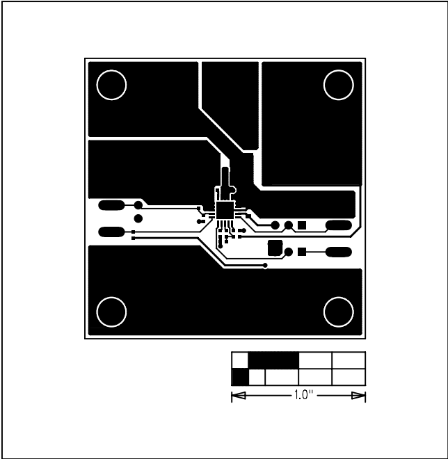
Figure 13. MAX17504 3.3V Output EV Kit Component Side PCB layout
