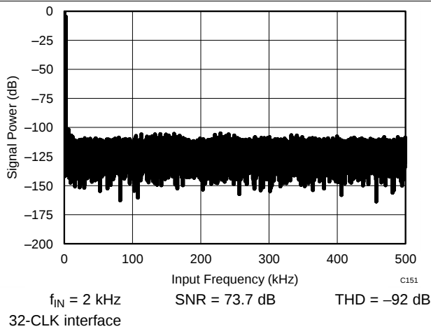
Figure 54. Typical FFT
