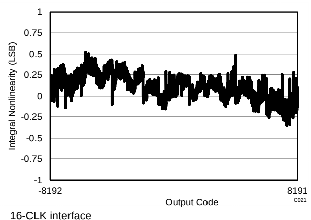
Figure 45. Typical INL
