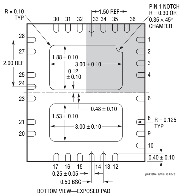
BOTTOM VIEW—EXPOSED PAD
