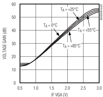
IF VGA VOLTAGE GAIN vs. IF VGA
