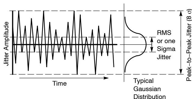
Figure 9. Peak-to-Peak Jitter
