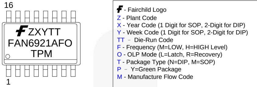
Figure 3. Marking Diagram
