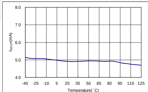
Figure 10. Operating Current
