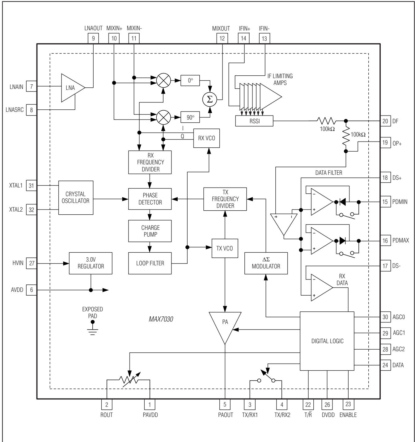
Functional Diagram
