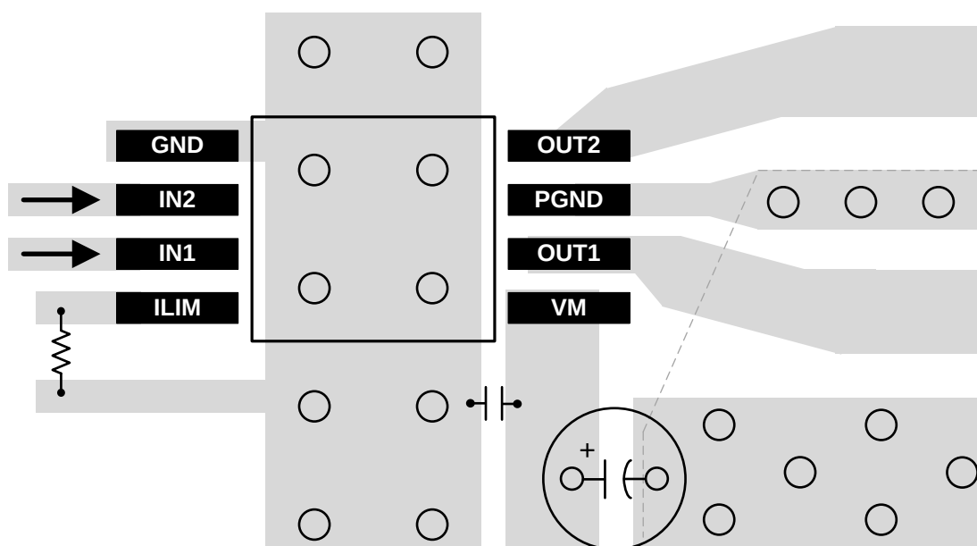
Figure 15. Layout Recommendation
