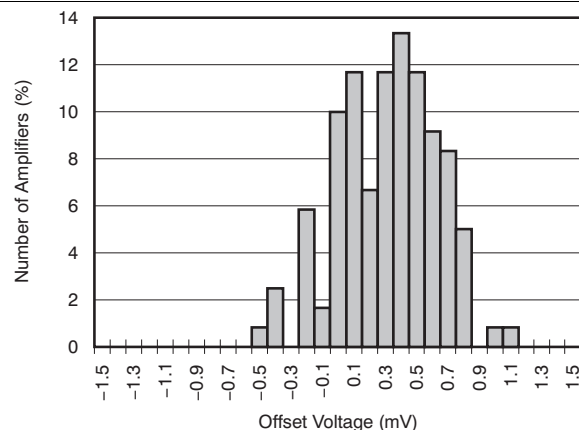
Figure 7. Offset Voltage Production Histogram
