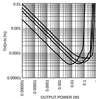
Figure 8. THD+N vs Output Power LME49720/LME49600 headphone amplifier into (from top to bottom at 10mW): 16Ω, 32Ω, 64Ω, 300Ω ( V_s = \pm 9V , f = 100\text{Hz} , 22\text{Hz} \leq \text{BW} \leq 22\text{kHz} )
