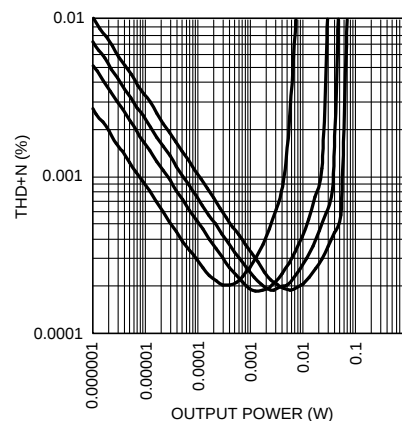
Figure 10. THD+N vs Output Power LME49720/LME49600 headphone amplifier into (from top to bottom at 0.1mW): 16Ω, 32Ω, 64Ω, 300Ω ( V_s = \pm 3V , f = 1\text{kHz} , 400\text{Hz} \leq \text{BW} \leq 22\text{kHz} )
