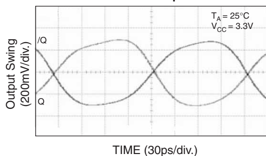
4GHz Output
