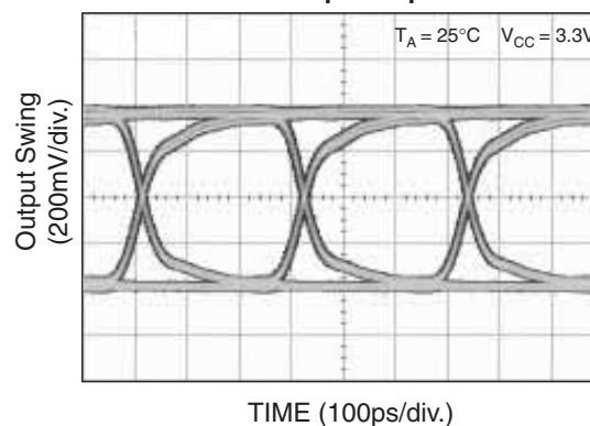
3.2Gbps Output
