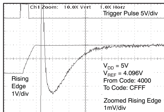
Figure 15. Half-Scale Settling Time: Rising Edge
