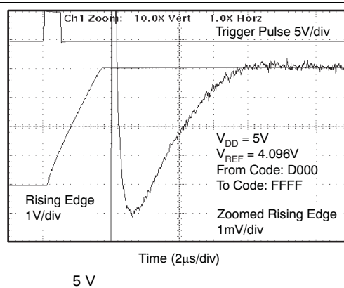
Figure 13. Full-Scale Settling Time: Rising Edge
